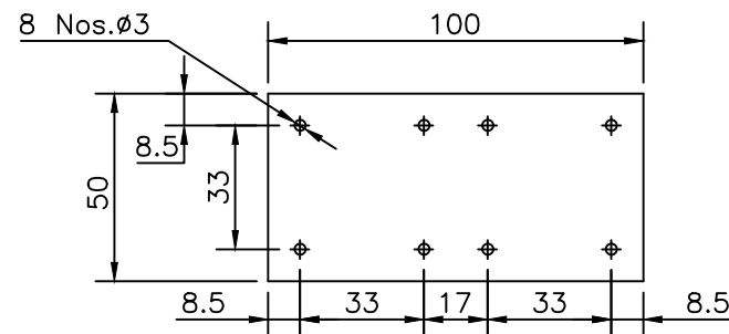
SUPPORT PLATE
